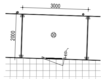
Berging 1:100
